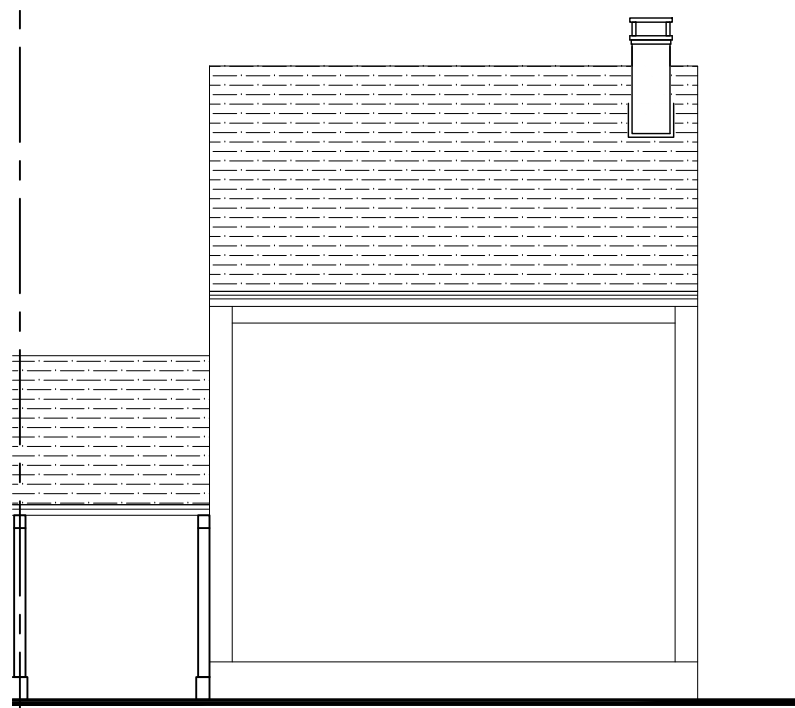
FACADE ARRIERE
